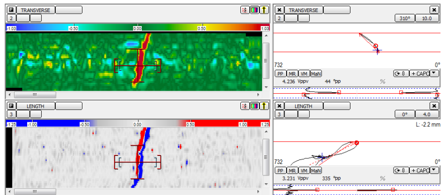
Transverse crack
