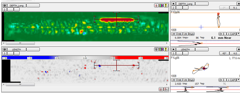
Longitudinal crack approx. 6 mm (¼in) deep, 78 mm (3in) long
