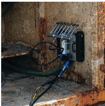
Custom Payloads: Inuktun MiniMag™ with specialized AquaTech Aqua-Cavi cleaning system
